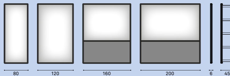
whiteboard + upholstered panel / oak decor panel / Whiteboard + gepolstertes Paneel / Eiche Dekor Paneel
